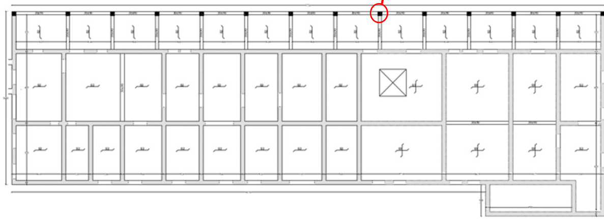
Fig.3. Pilastro in c.a. corpo 6, piano terra fronte Ovest.
